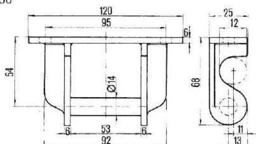
CERNIERA SPONDA ALL. 25 Cod. 09.0320 gr. 360
