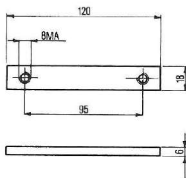
PIASTRINA INTER. 95 Cod. 09.0316 gr. 100
