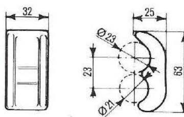
PALETTA Cod. 09.0328 gr. 25
