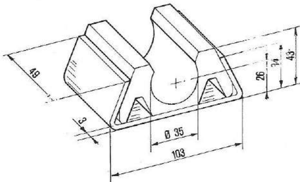
SUPPORTO IN GOMMA TUBO CENTINA Cod. 07.0310 gr. 295
