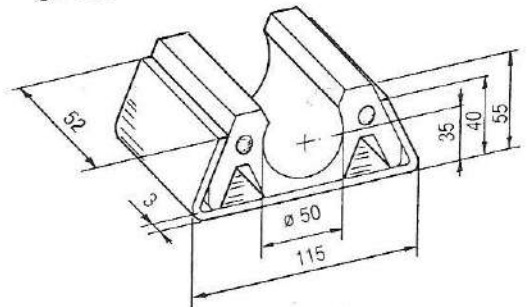
SUPPORTO IN GOMMA TUBO CENTINA Cod. 07.0312 gr. 365
