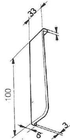
SUPPORTO IN GOMMA TUBO CENTINA Cod. 07.0312 gr. 365
